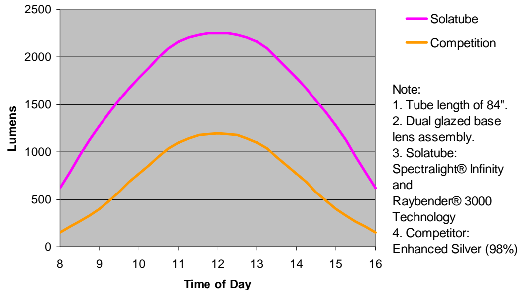
A Comparison of Hourly Lumen Performance for a Typical Winter Day in Mid-America (Denver) With a 14" Diameter Tube
